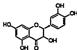
TAXIFOLIN
